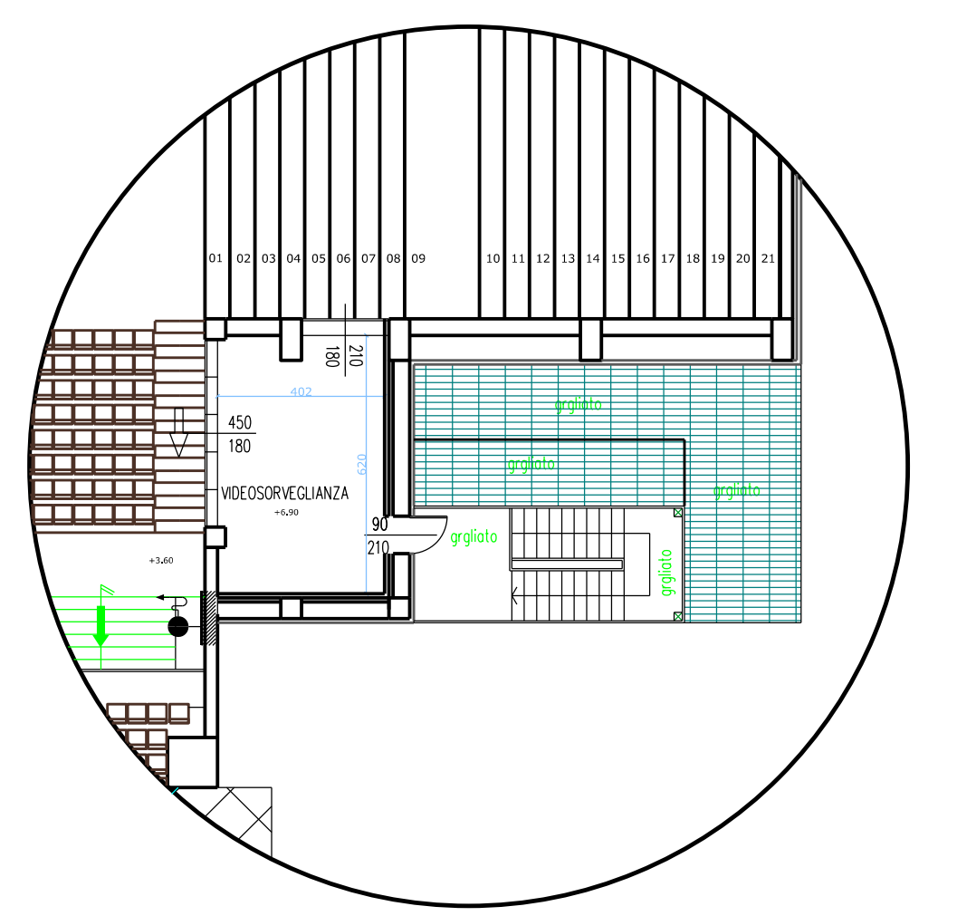
PARTIC. P.SECONDO
